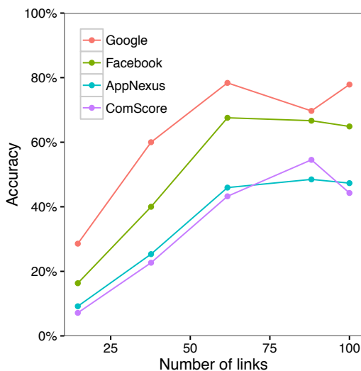
Figure 8: De-anonymization accuracy on the subset of links visible to various organizations that track online behavior, based on user-submitted histories.
